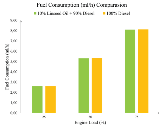
Fig. 3. Variation in engine fuel consumption according to load and fuel type
