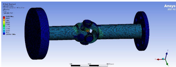
Figure 4. Stress in the shaft model under boundary conditions.
