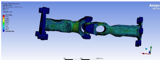
Figure 9. Stress in the optimized shaft model under boundary conditions.
