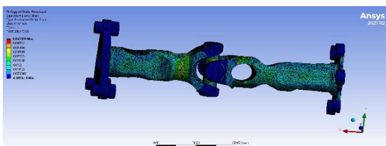
Figure 10. Strain in the optimized shaft model under boundary conditions.
