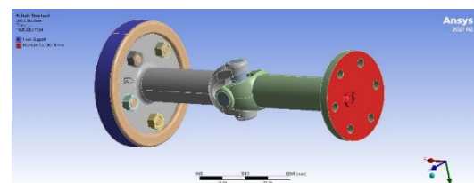
Figure 3. Boundary conditions applied to the shaft.
