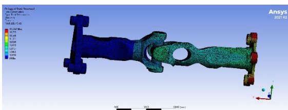
Figure 11. Deformation in the optimized shaft model under boundary conditions.
