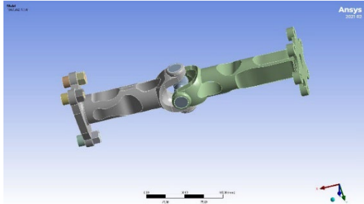
Figure 8. The redesigned model according to the optimized model.
