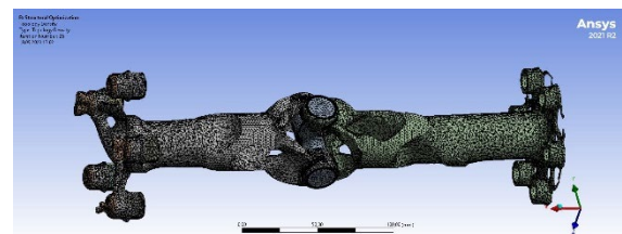
Figure 7. Optimized shaft model.
