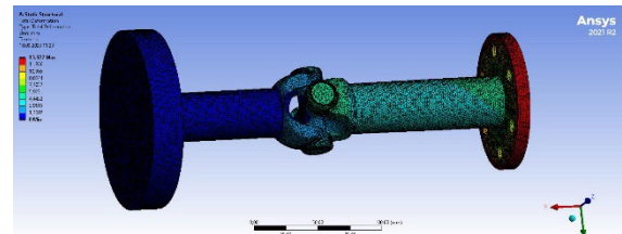
Figure 6. Deformation in the shaft model under boundary conditions.
