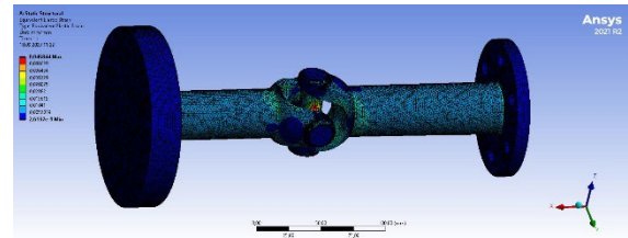
Figure 5. Strain in the shaft model under boundary conditions.
